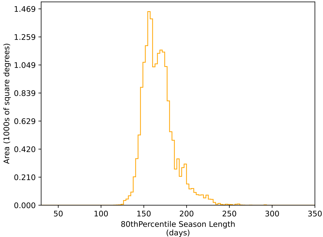
internal_u_expt38_nscale1.5v3.4_10yrs WFD r band: 80thPercentile Season Length
