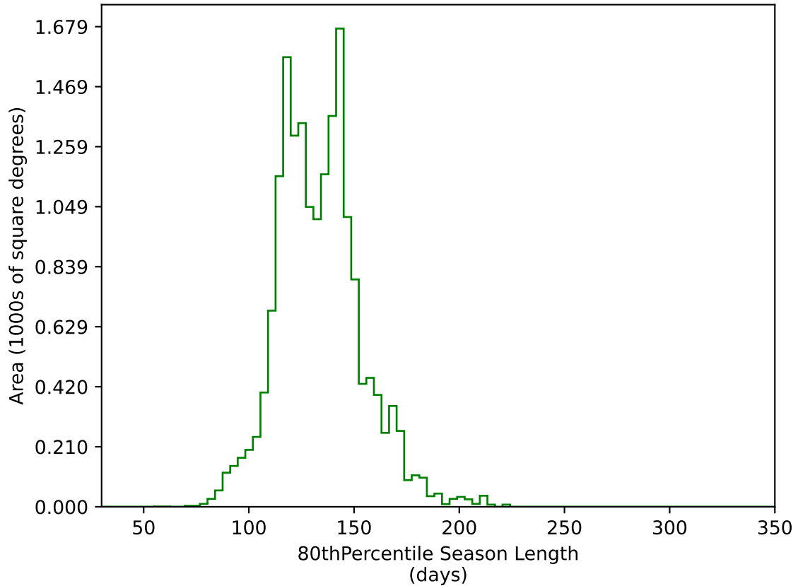
internal_u_expt38_nscale1.5v3.4_10yrs WFD g band: 80thPercentile Season Length
