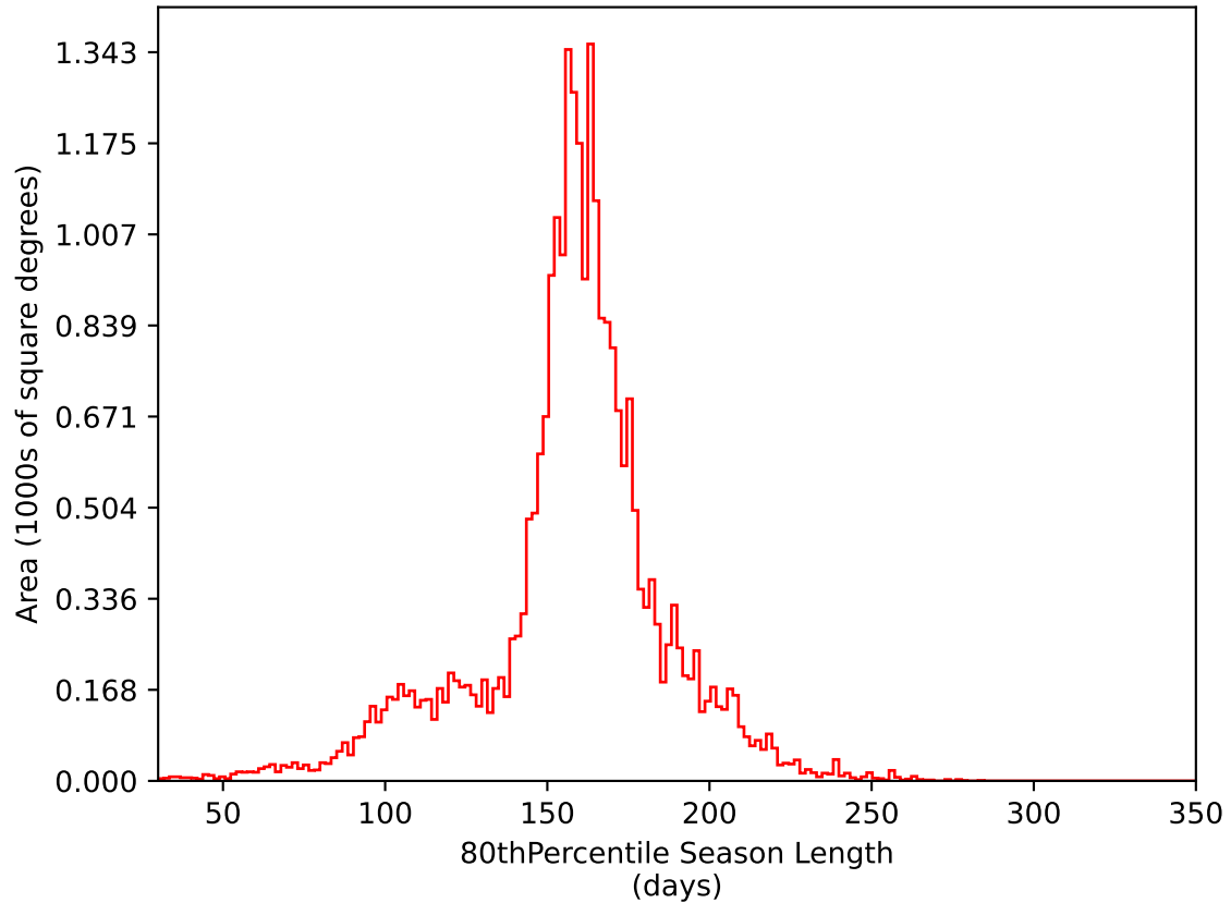
internal_u_expt38_nscale1.5v3.4_10yrs All sky i band: 80thPercentile Season Length
