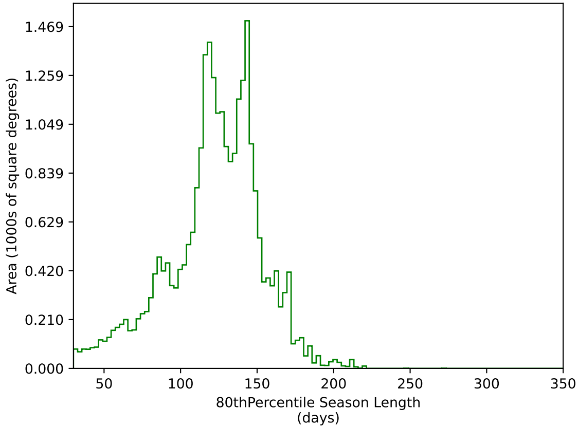
internal_u_expt38_nscale1.5v3.4_10yrs All sky g band: 80thPercentile Season Length
