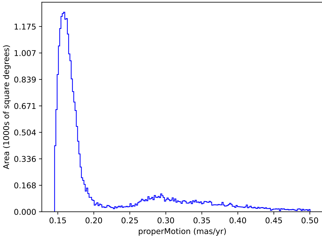
internal_u_expt38_nscale1.5v3.4_10yrs : properMotion
