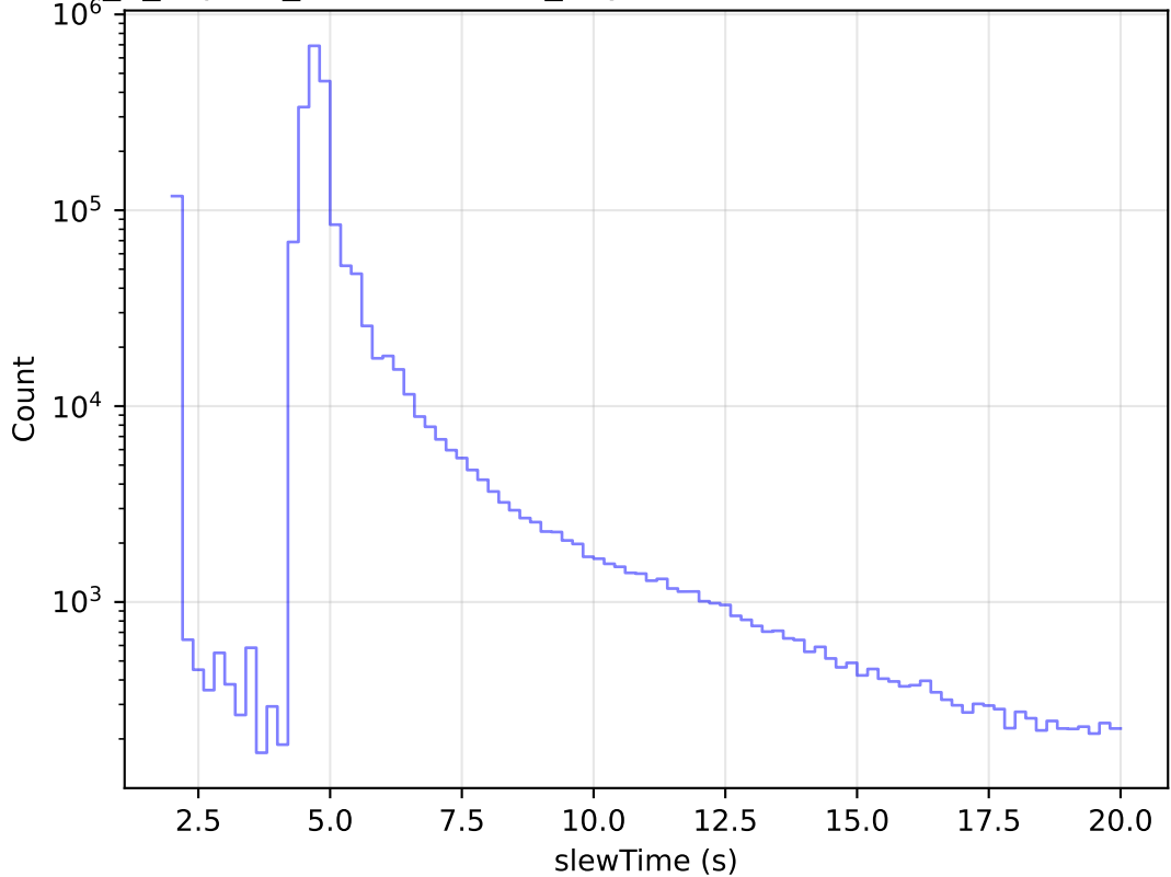
internal_u_expt38_nscale1.5v3.4_10yrs All visits: Zoom Slew Time Histogram
