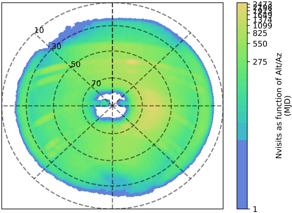
internal_u_expt38_nscale1.5v3.4_10yrs z: Nvisits as function of Alt/Az
