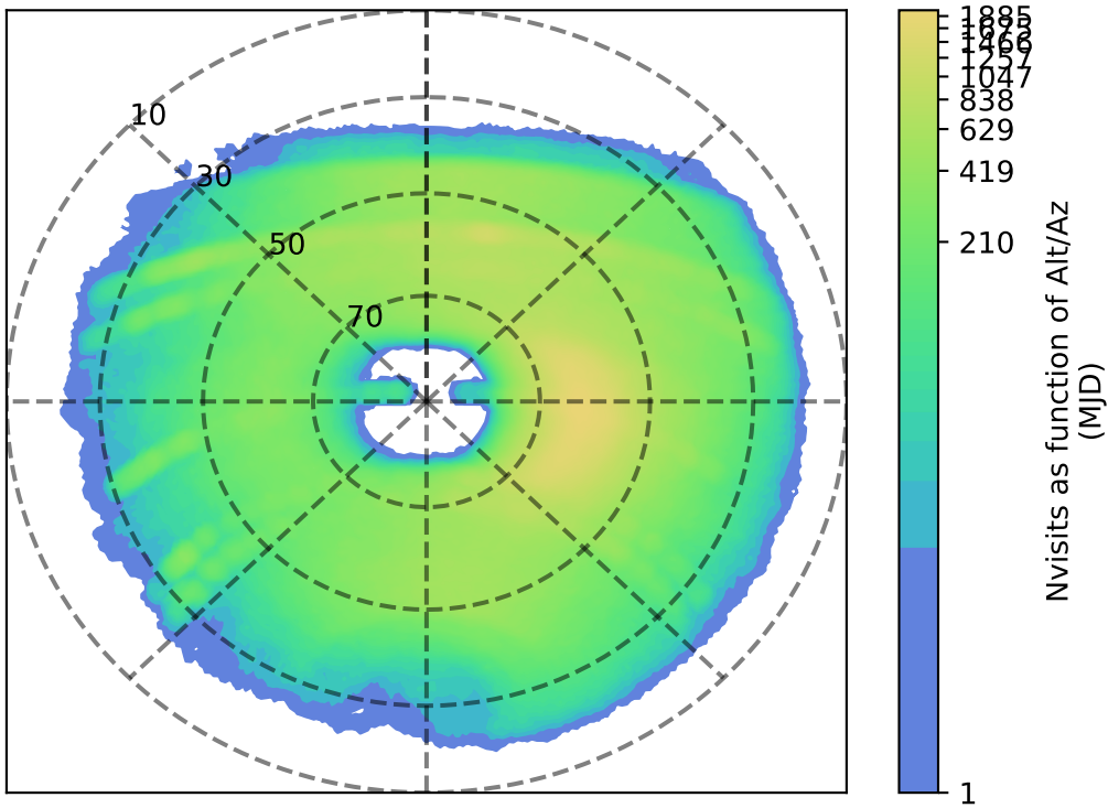
internal_u_expt38_nscale1.5v3.4_10yrs y: Nvisits as function of Alt/Az
