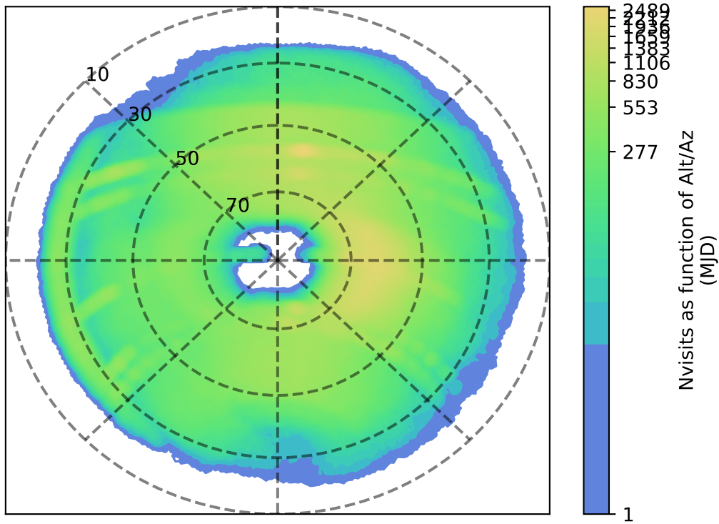
internal_u_expt38_nscale1.5v3.4_10yrs r: Nvisits as function of Alt/Az
