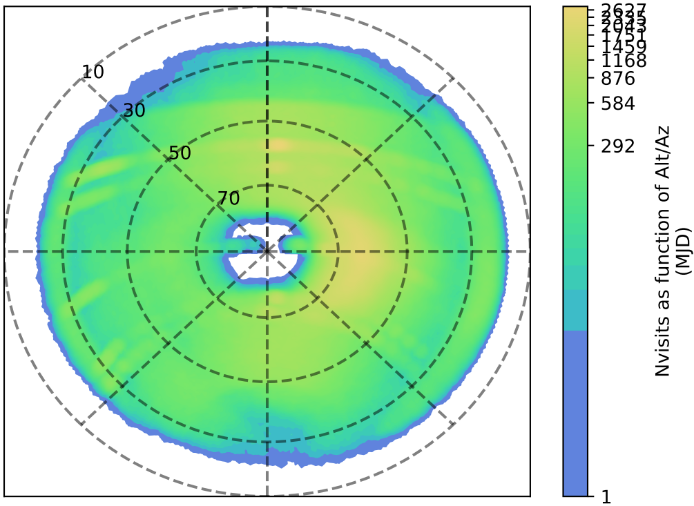
internal_u_expt38_nscale1.5v3.4_10yrs i: Nvisits as function of Alt/Az
