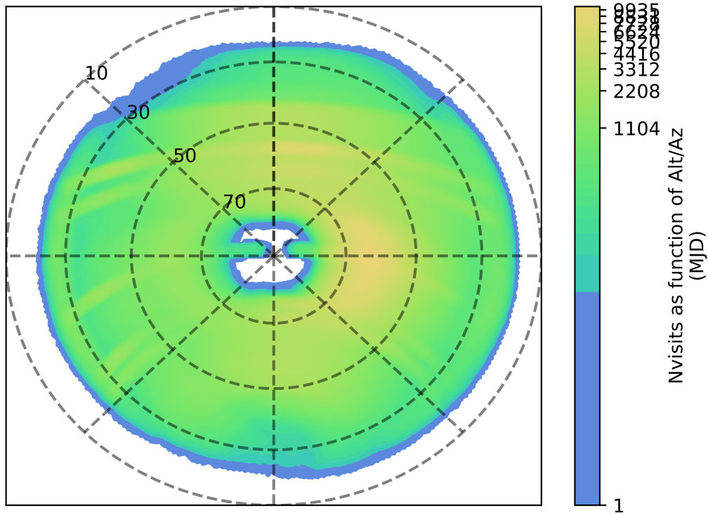
internal_u_expt38_nscale1.5v3.4_10yrs : Nvisits as function of Alt/Az
