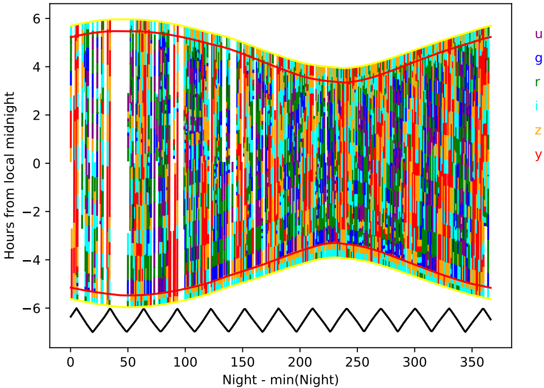
internal_u_expt38_nscale1.5v3.4_10yrs year 6-7: Hourglass
