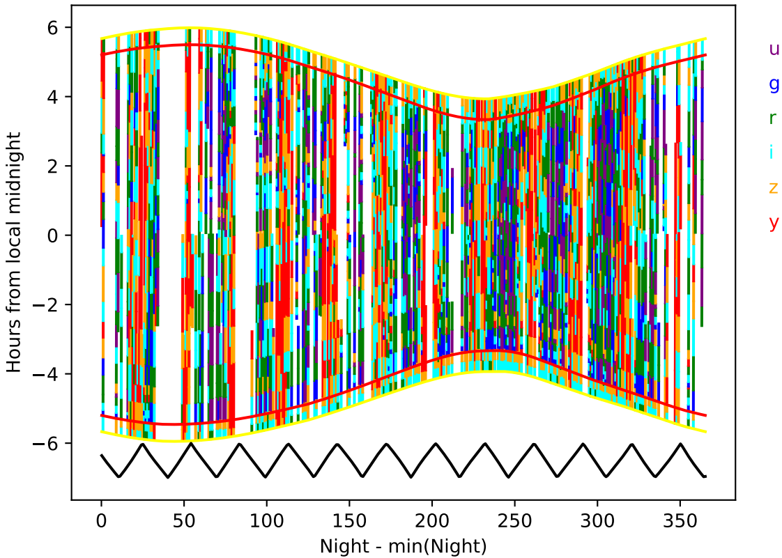
internal_u_expt38_nscale1.5v3.4_10yrs year 4-5: Hourglass
