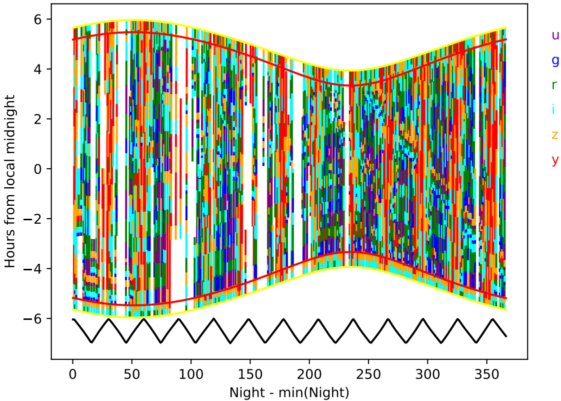
internal_u_expt38_nscale1.5v3.4_10yrs year 1-2: Hourglass
