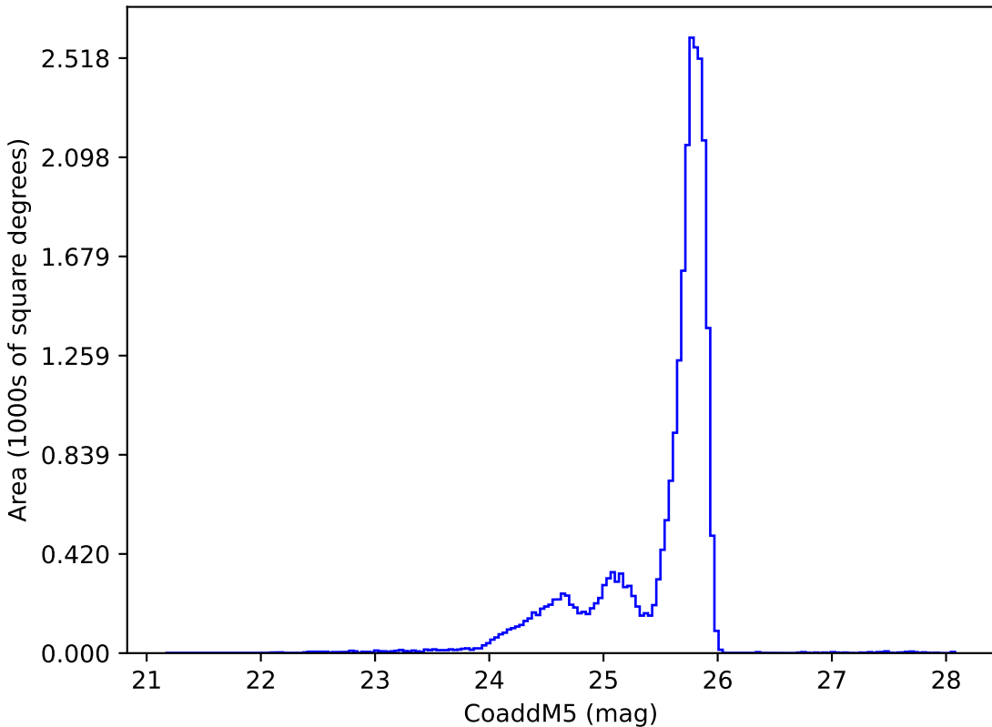
internal_u_expt38_nscale1.5v3.4_10yrs z: CoaddM5
