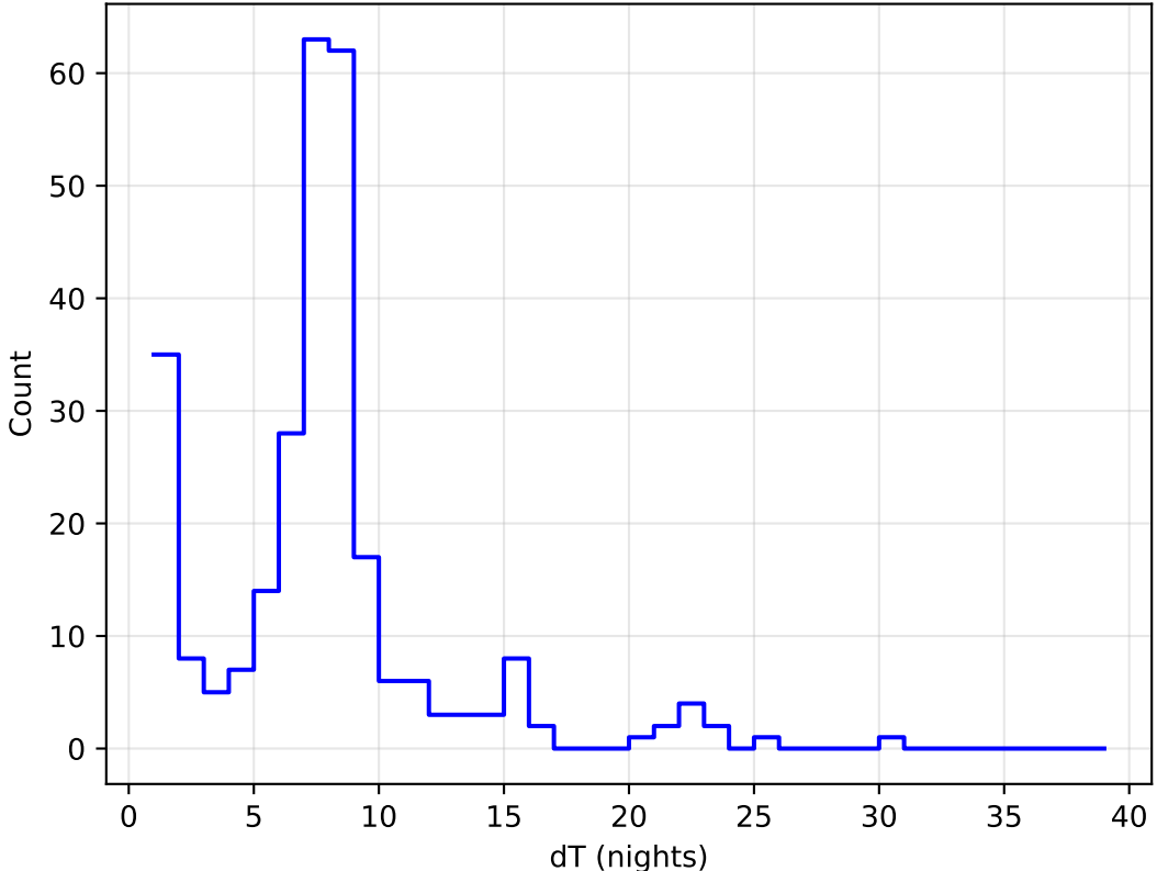
internal_u_expt38_nscale1.5v3.4_10yrs all bands: DD:ECDFS Delta Nights Histogram
