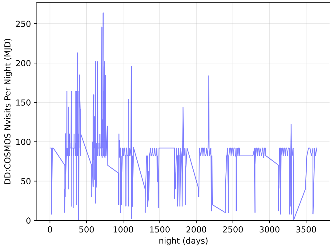
internal_u_expt38_nscale1.5v3.4_10yrs all bands: DD: COSMOS Nvisits Per Night
