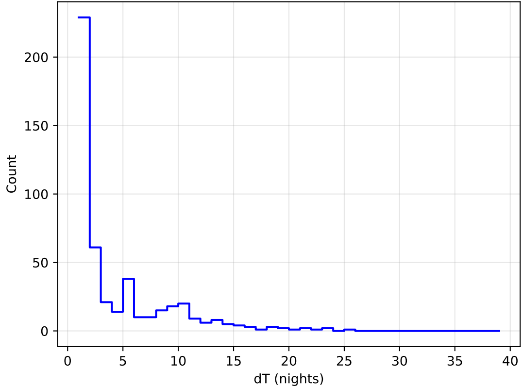
internal_u_expt38_nscale1.5v3.4_10yrs all bands: DD: COSMOS Delta Nights Histogram
