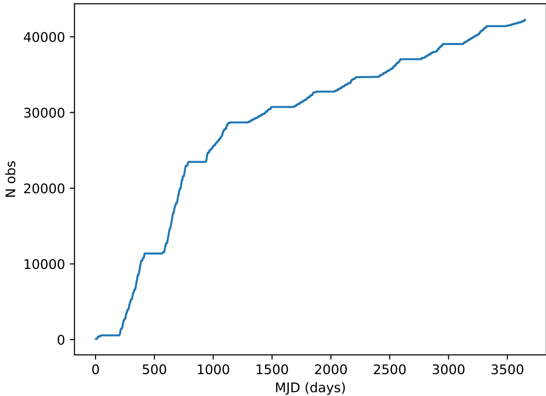
internal_u_expt38_nscale1.5v3.4_10yrs all bands: DD: COSMOS Cumulative NVisits
