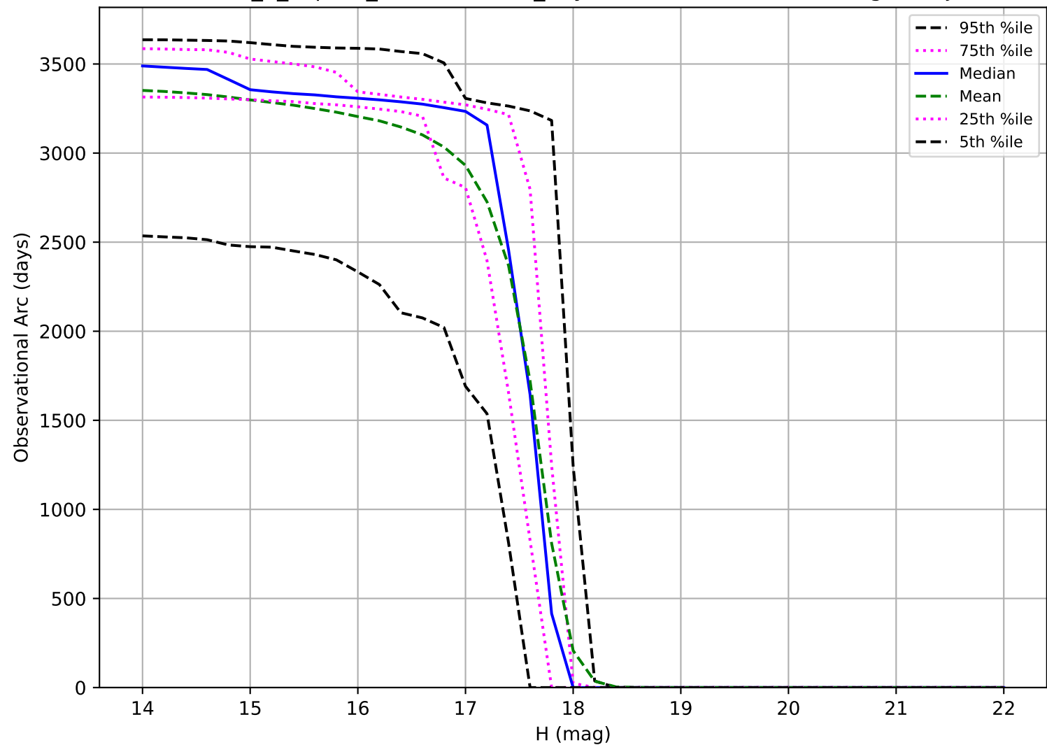
internal_u_expt38_nscale1.2v3.4_10yrs: Observational Arc Length Trojan
