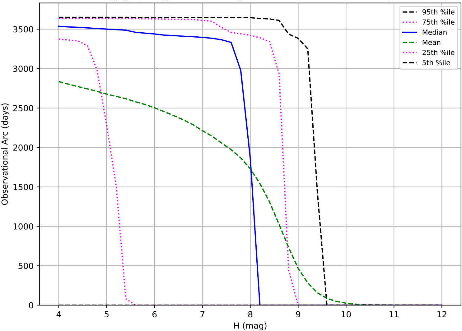
internal_u_expt38_nscale1.2v3.4_10yrs: Observational Arc Length TNO
