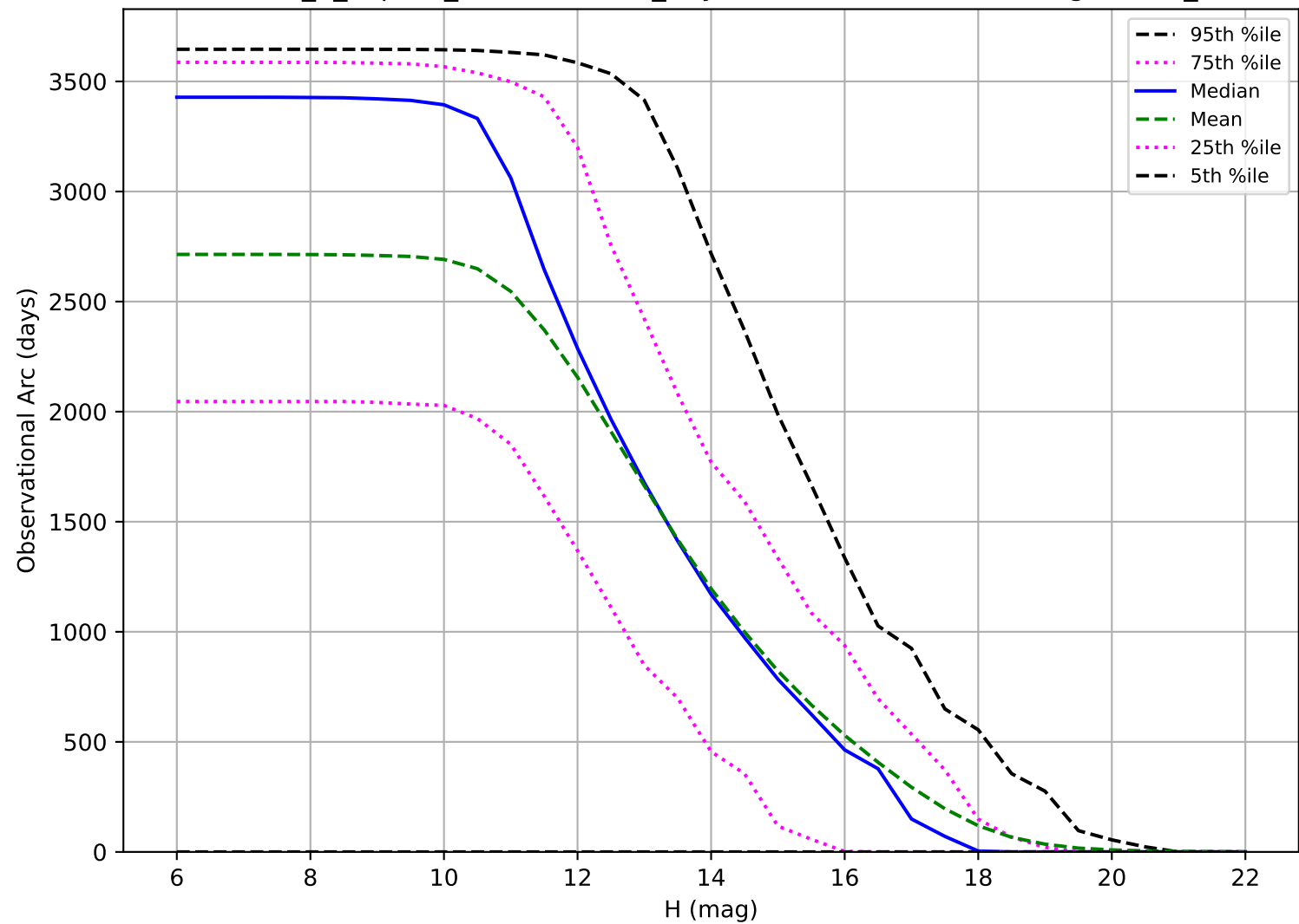
internal_u_expt38_nscale1.2v3.4_10yrs: Observational Arc Length OCC_r5
