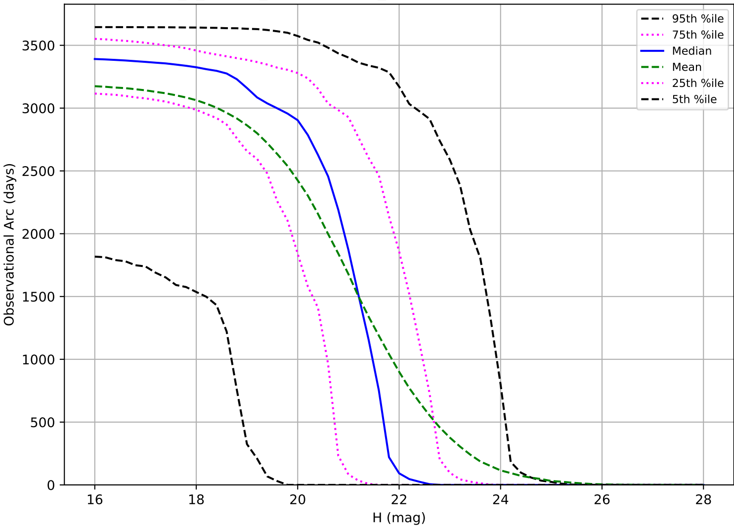
internal_u_expt38_nscale1.2v3.4_10yrs: Observational Arc Length NEO
