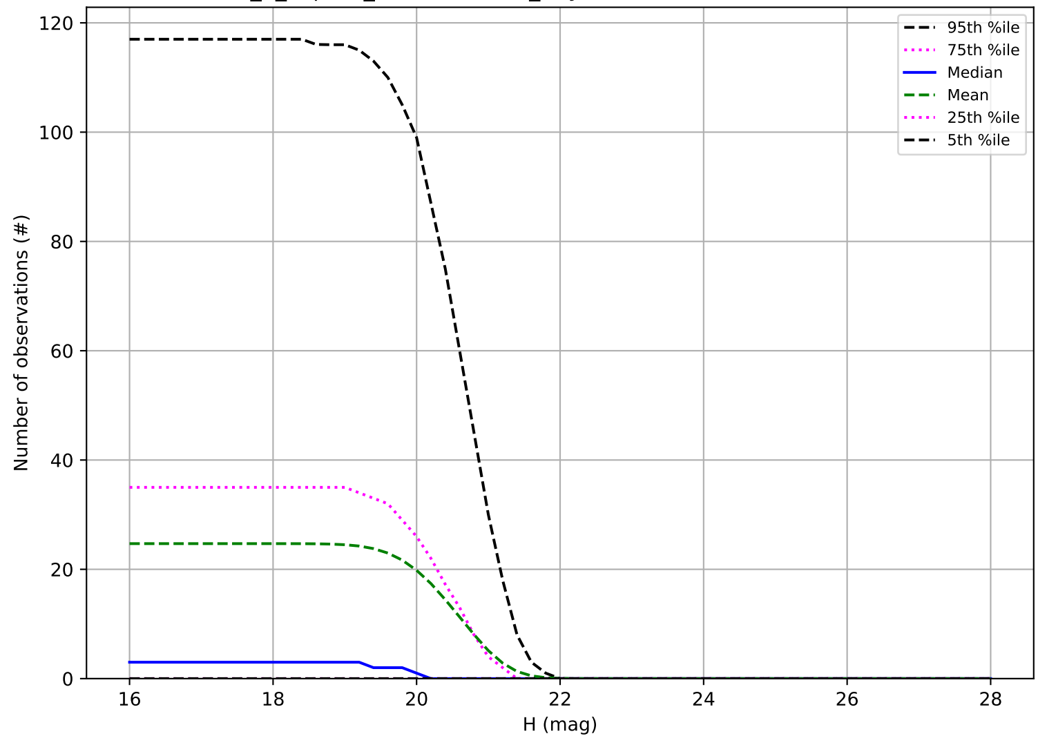
internal_u_expt38_nscale1.2v3.4_10yrs: Number of observations Vatira
