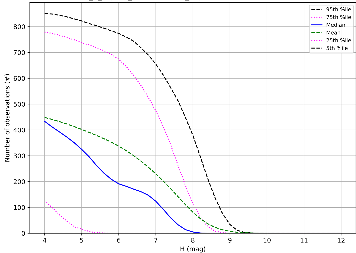
internal_u_expt38_nscale1.2v3.4_10yrs: Number of observations TNO
