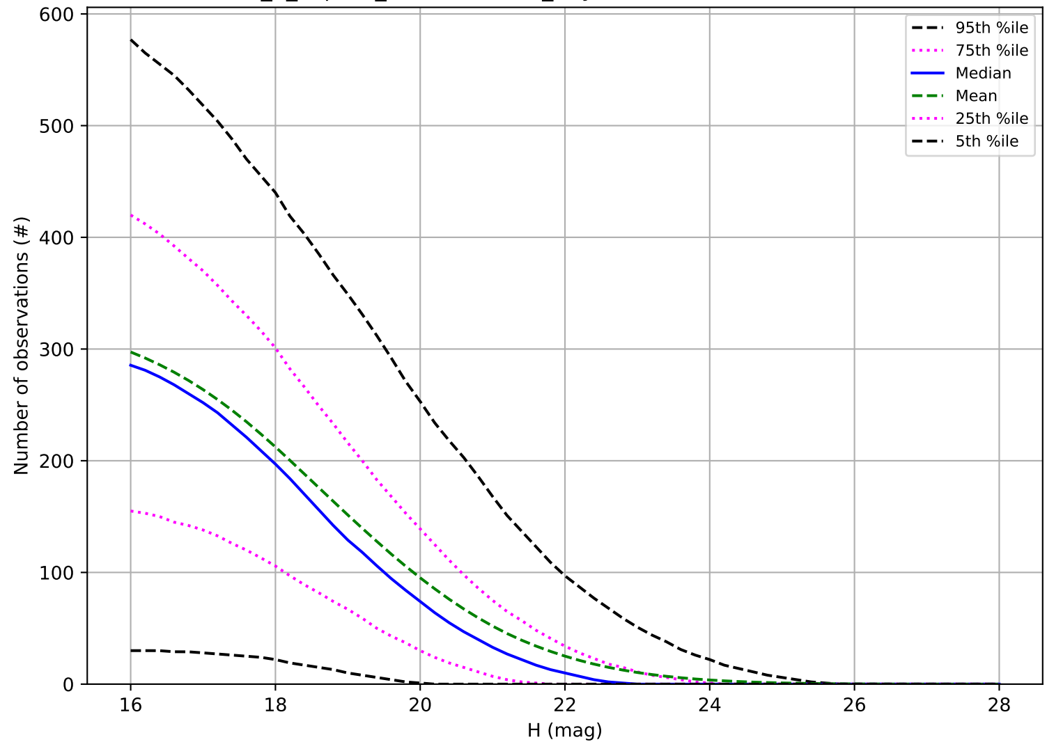
internal_u_expt38_nscale1.2v3.4_10yrs: Number of observations NEO
