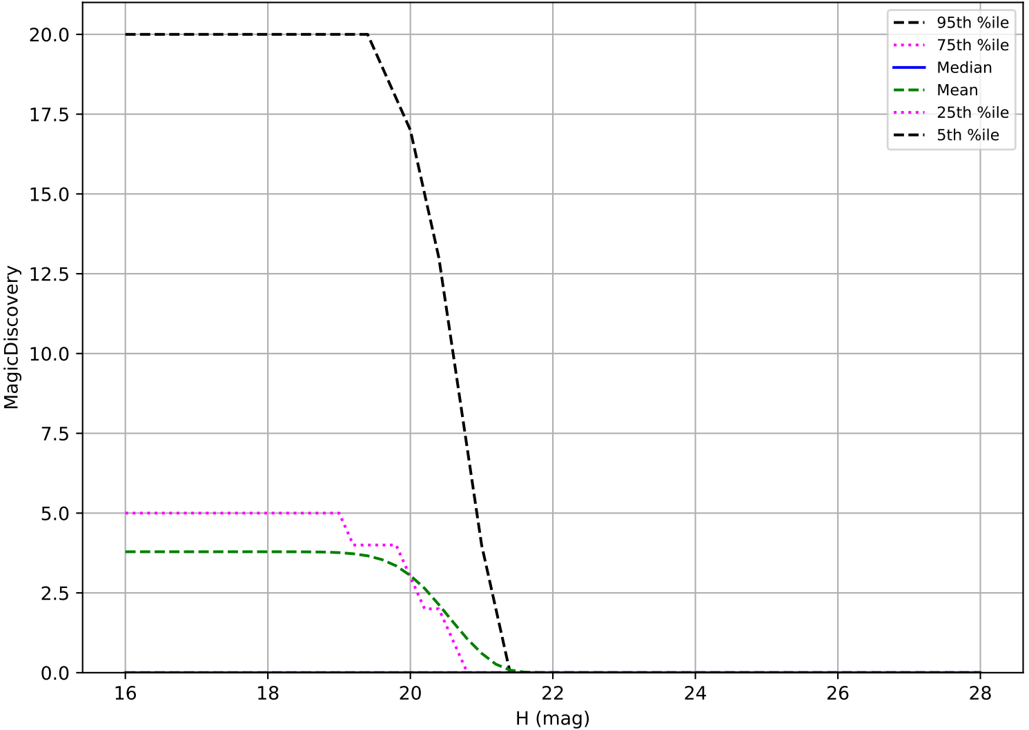
internal_u_expt38_nscale1.2v3.4_10yrs: Vatira 6 detections in 60 nights detection loss
