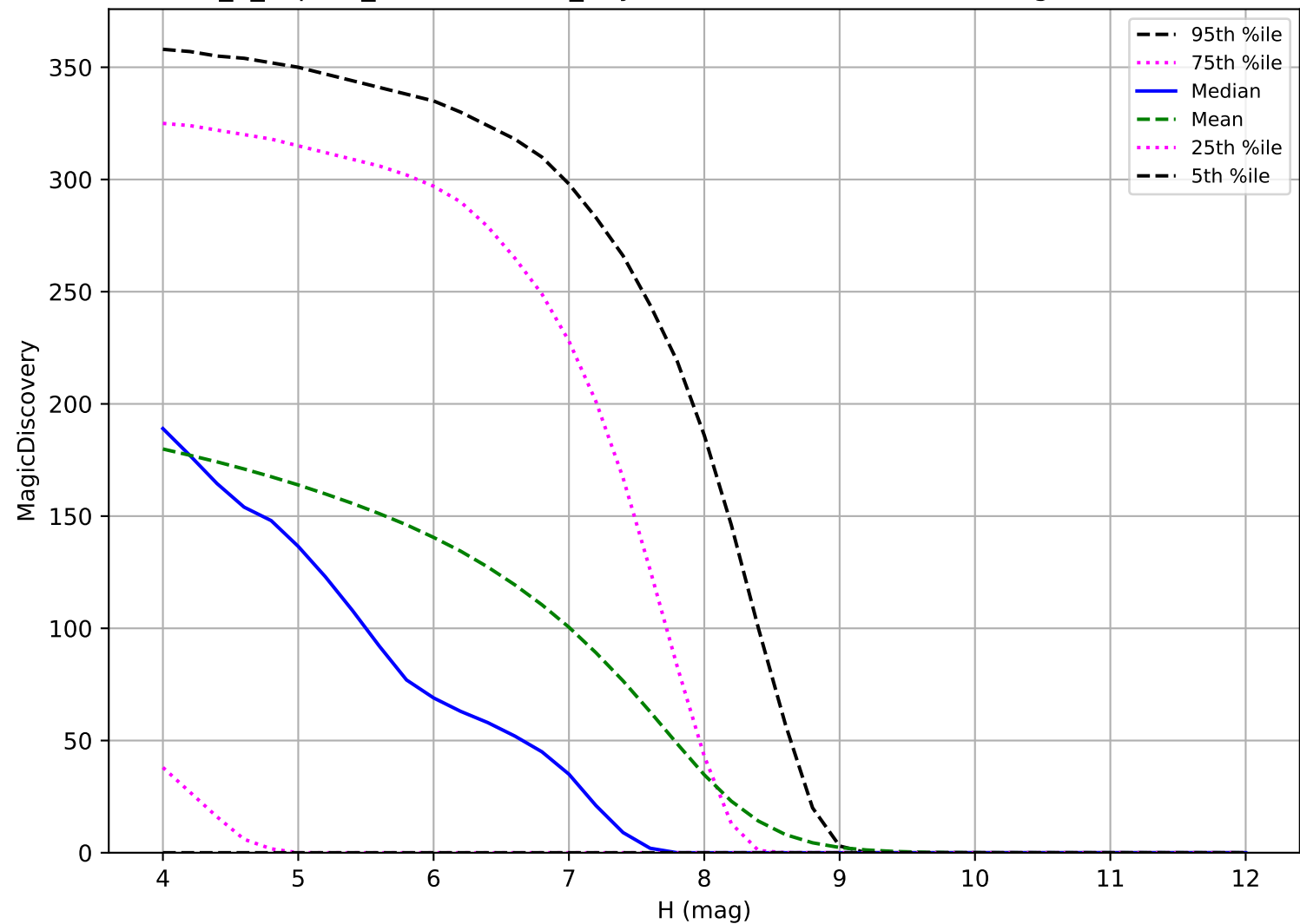
internal_u_expt38_nscale1.2v3.4_10yrs: TNO 6 detections in 60 nights detection loss
