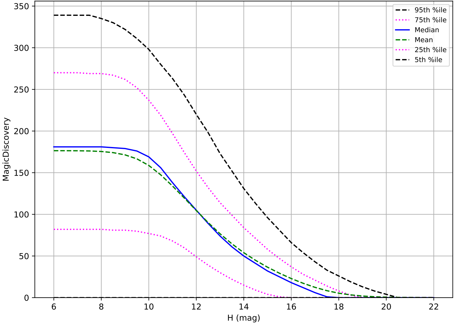
internal_u_expt38_nscale1.2v3.4_10yrs: OCC_r5 6 detections in 60 nights detection loss
