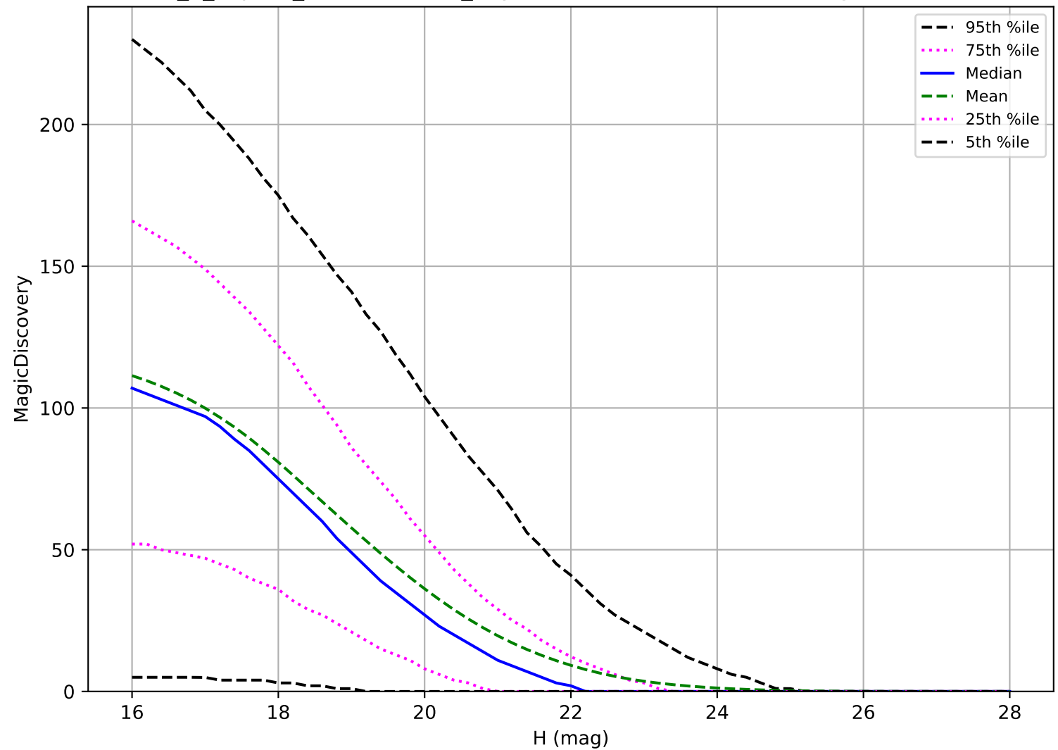
internal_u_expt38_nscale1.2v3.4_10yrs: NEO 6 detections in 60 nights detection loss
