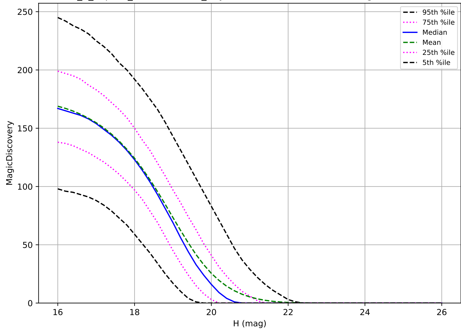
internal_u_expt38_nscale1.2v3.4_10yrs: MBA 6 detections in 60 nights detection loss
