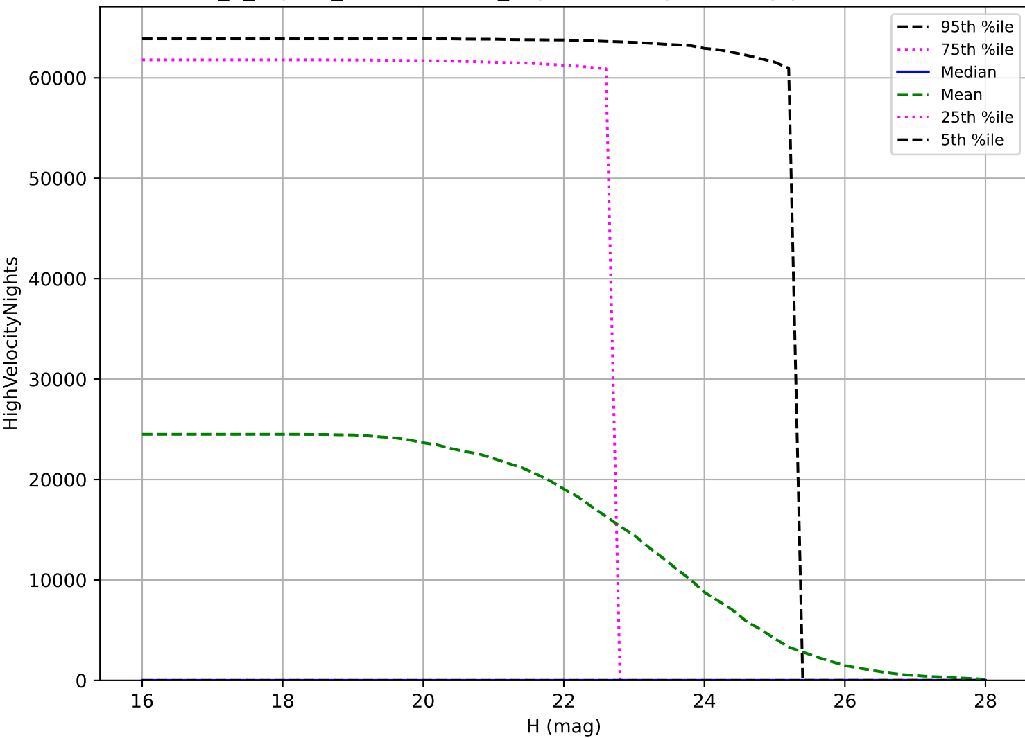
internal_u_expt38_nscale1.2v3.4_10yrs: PHA High velocity pair detection loss
