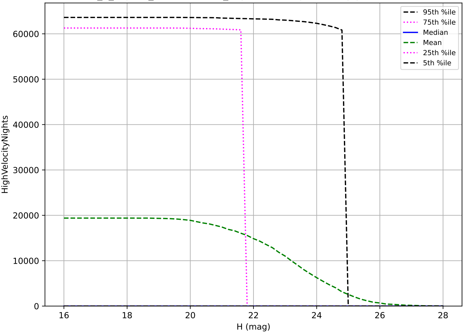
internal_u_expt38_nscale1.2v3.4_10yrs: NEO High velocity pair detection loss
