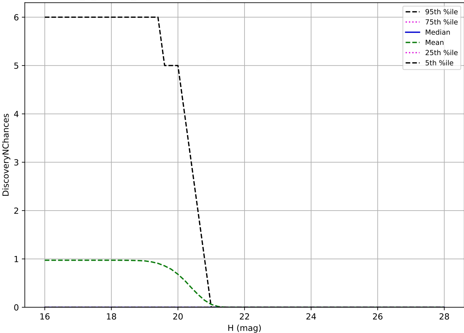
internal_u_expt38_nscale1.2v3.4_10yrs: Vatira 3 pairs in 15 nights detection loss
