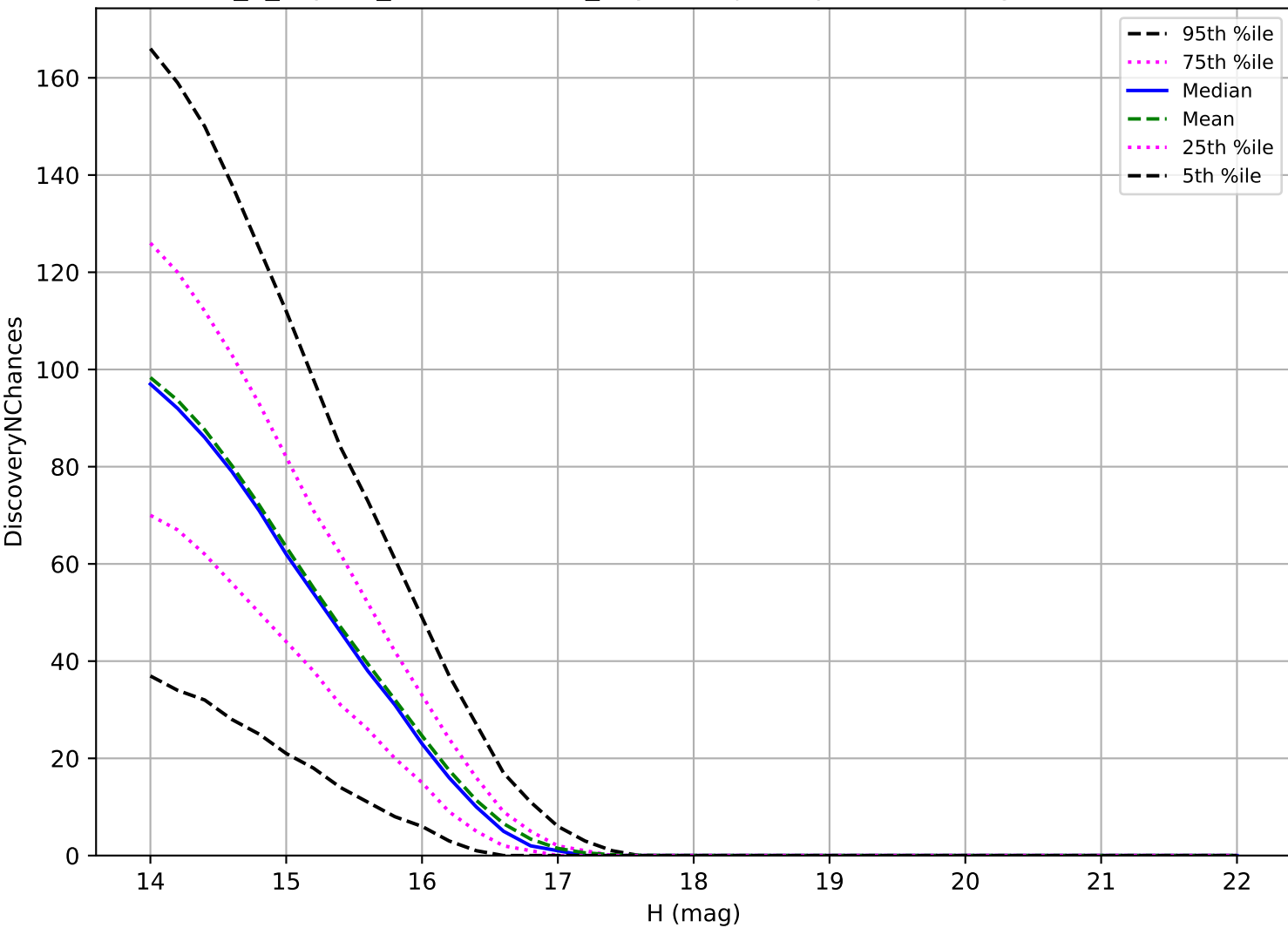
internal_u_expt38_nscale1.2v3.4_10yrs: Trojan 3 pairs in 15 nights detection loss
