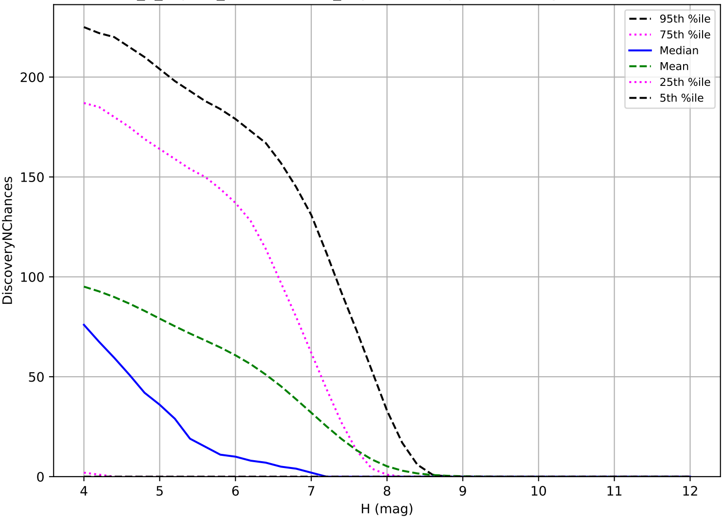
internal_u_expt38_nscale1.2v3.4_10yrs: TNO 3 pairs in 15 nights detection loss
