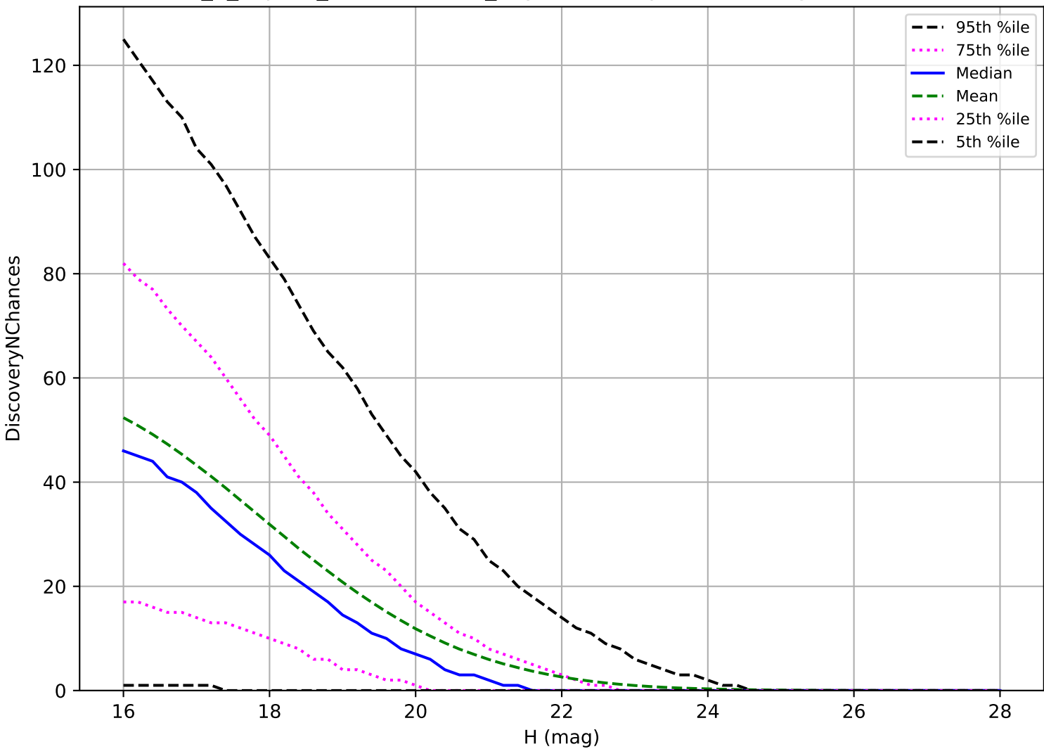
internal_u_expt38_nscale1.2v3.4_10yrs: PHA 3 pairs in 15 nights detection loss
