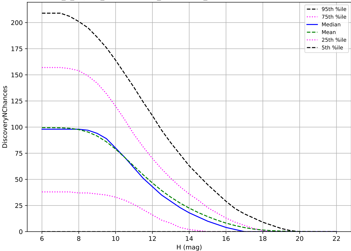
internal_u_expt38_nscale1.2v3.4_10yrs: OCC_r5 3 pairs in 15 nights detection loss
