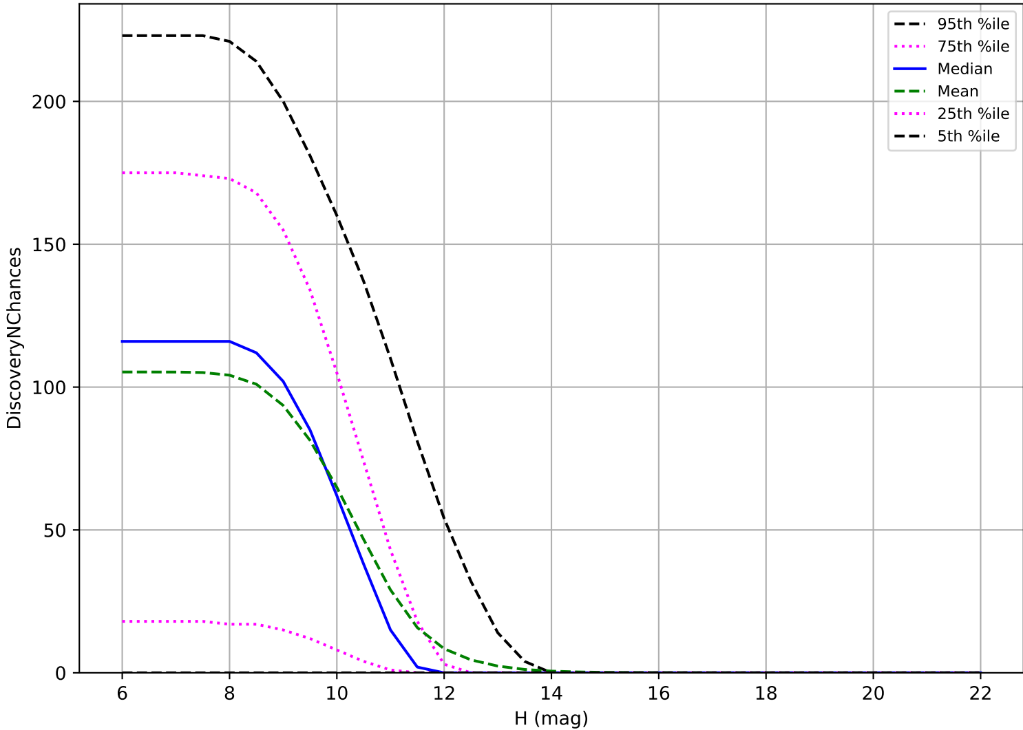
internal_u_expt38_nscale1.2v3.4_10yrs: OCC_r20 3 pairs in 15 nights detection loss
