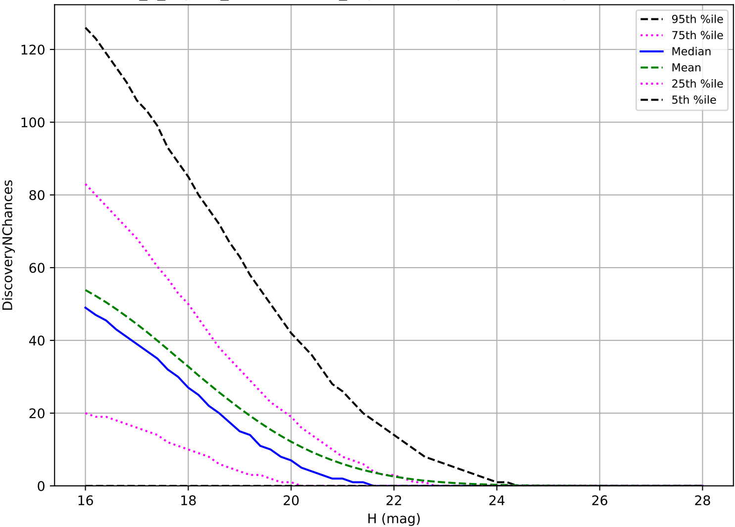
internal_u_expt38_nscale1.2v3.4_10yrs: NEO 3 pairs in 15 nights detection loss
