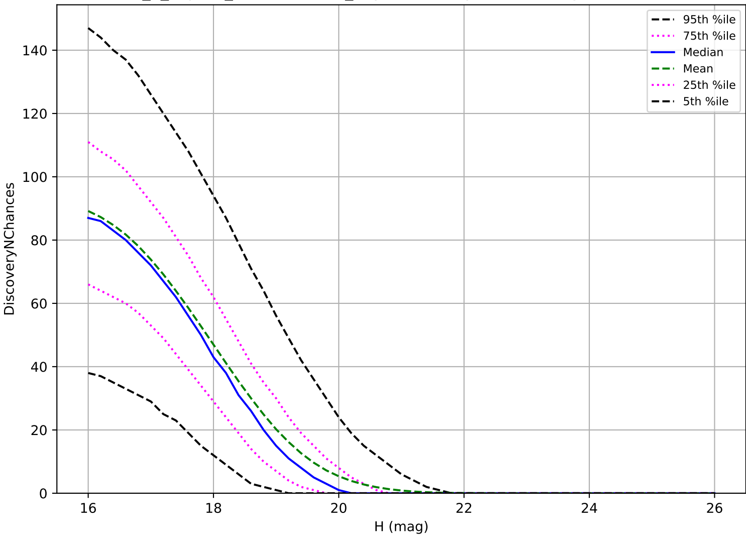
internal_u_expt38_nscale1.2v3.4_10yrs: MBA 3 pairs in 15 nights detection loss
