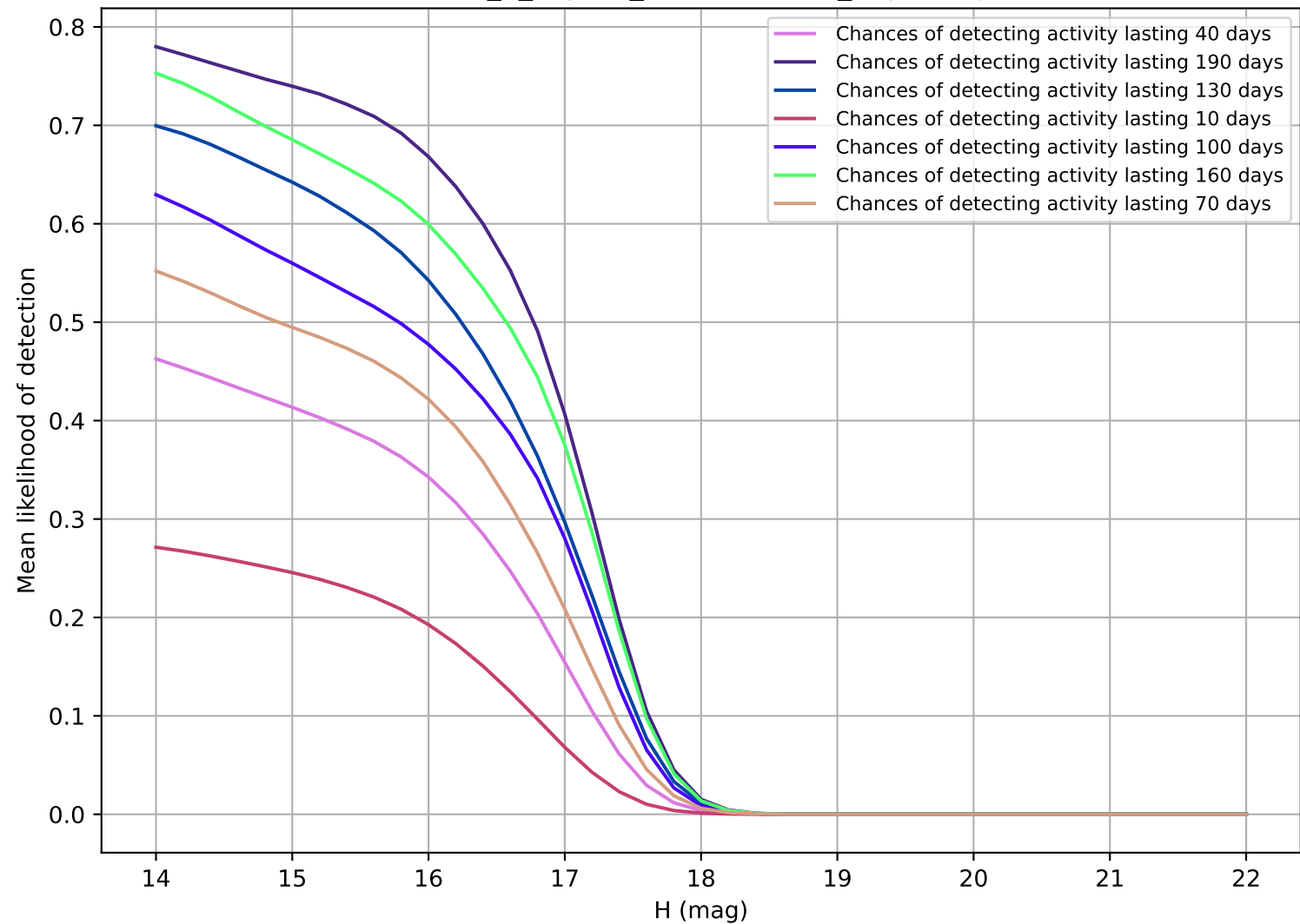
internal_u_expt38_nscale1.2v3.4_10yrs Trojan
