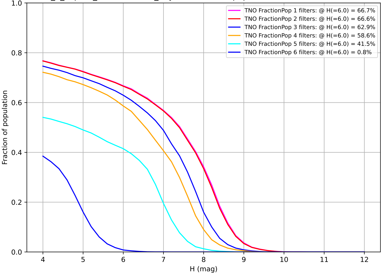
internal_u_expt38_nscale1.2v3.4_10yrs: Fraction of population with colors in X filters TNO
