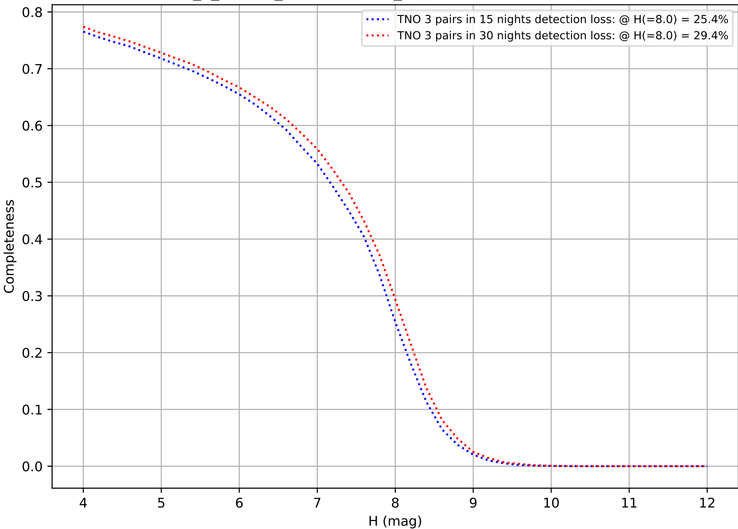
internal_u_expt38_nscale1.2v3.4_10yrs: DifferentialCompleteness
