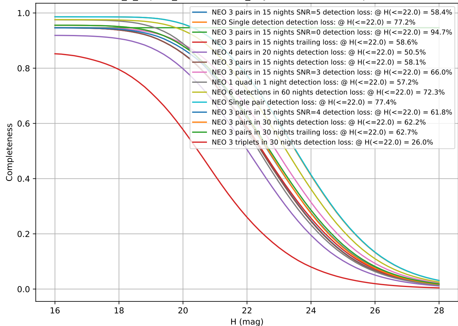
internal_u_expt38_nscale1.2v3.4_10yrs: CumulativeCompleteness
