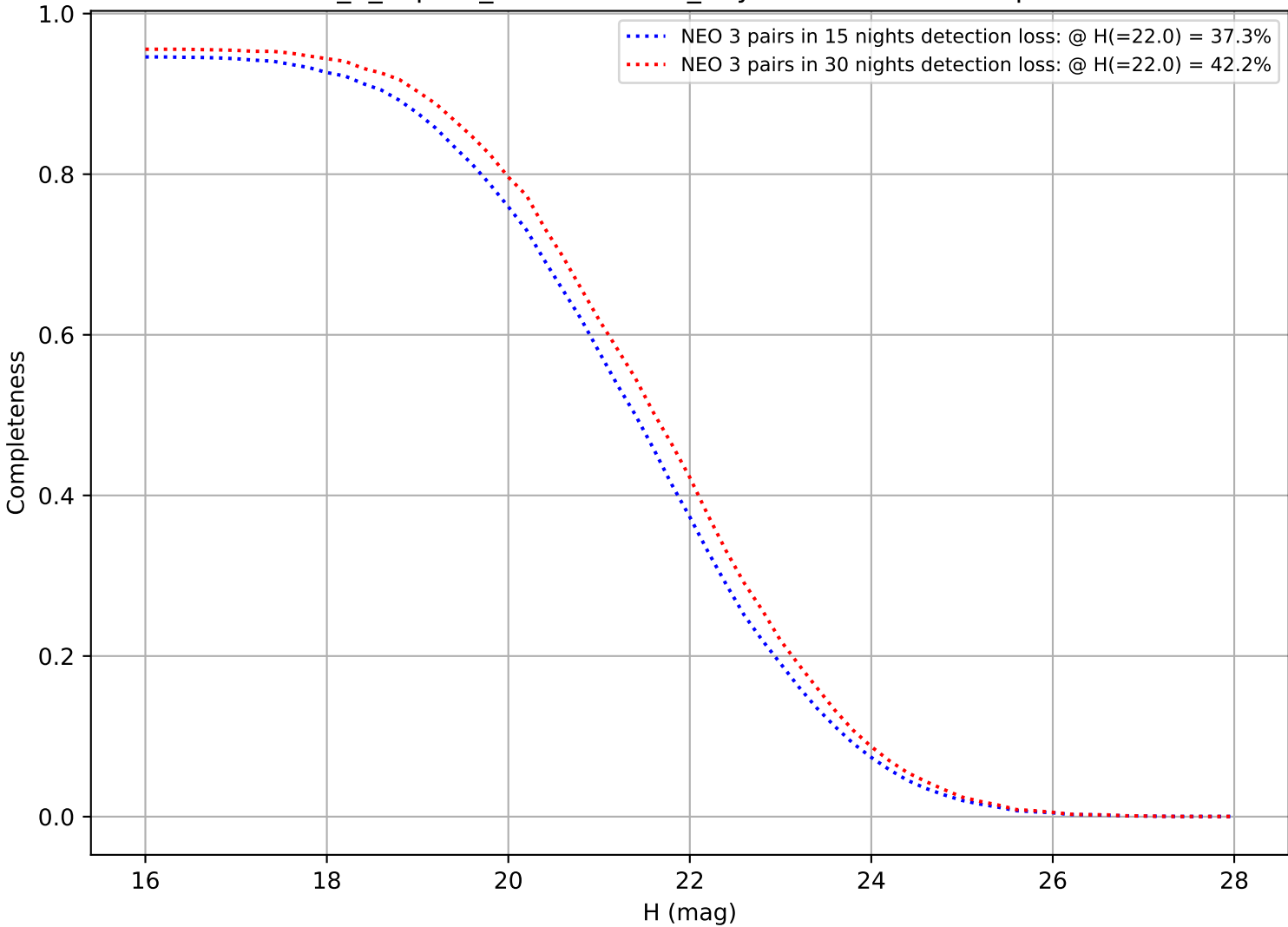
internal_u_expt38_nscale1.2v3.4_10yrs: DifferentialCompleteness
