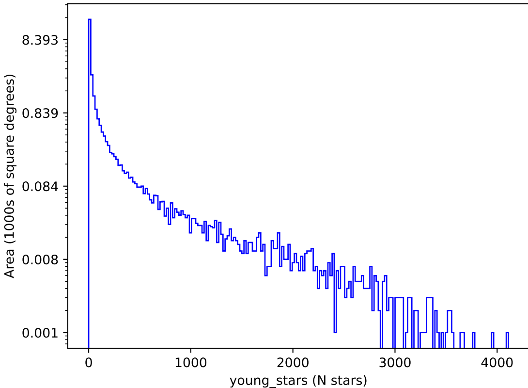
internal_u_expt38_nscale1.2v3.4_10yrs : young_stars
