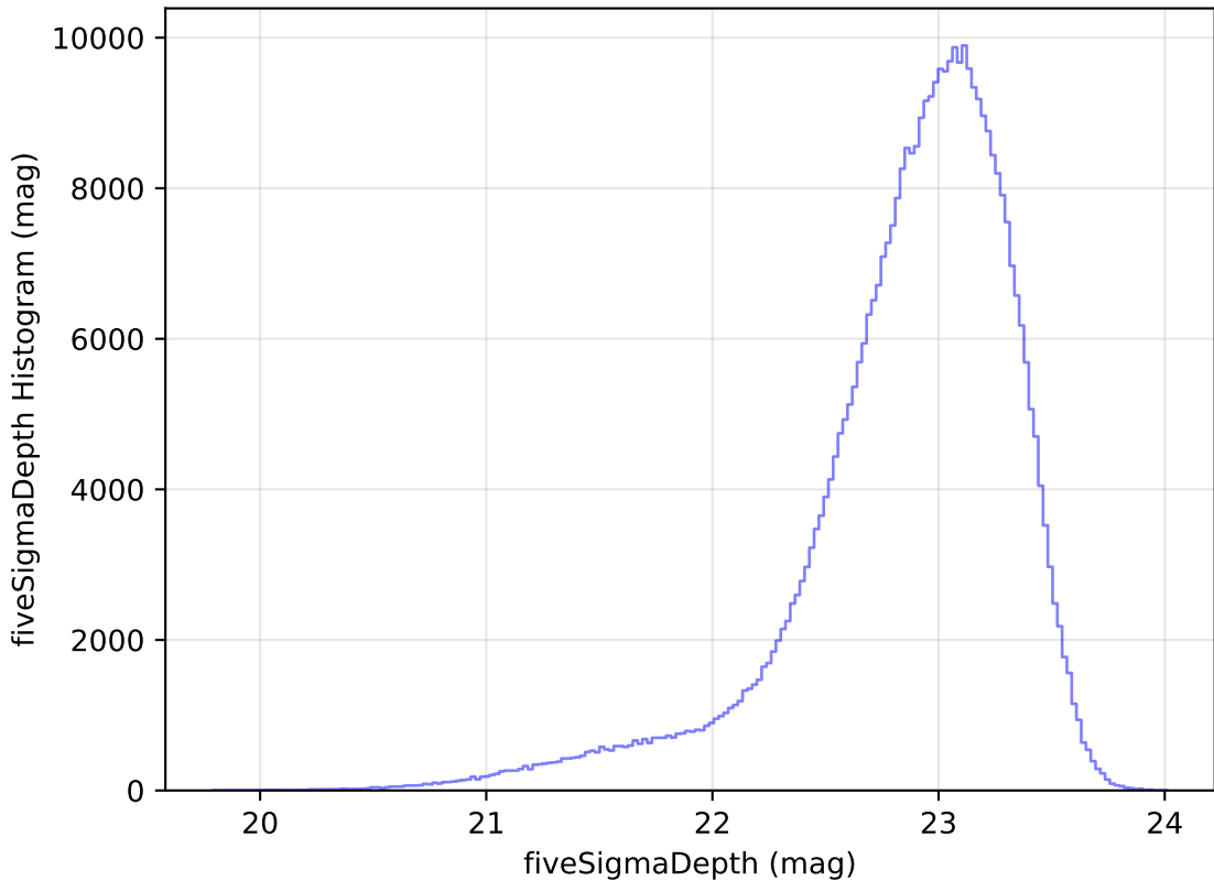
internal_u_expt38_nscale1.2v3.4_10yrs z: fiveSigmaDepth Histogram
