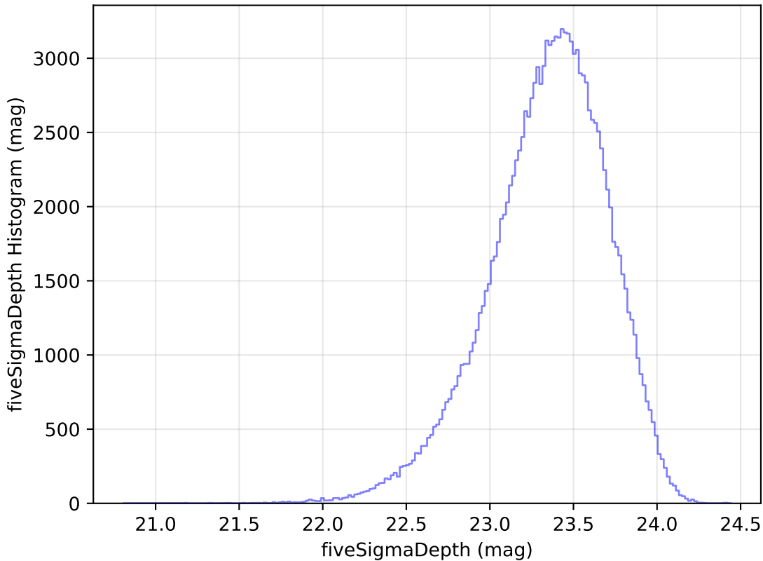
internal_u_expt38_nscale1.2v3.4_10yrs u: fiveSigmaDepth Histogram
