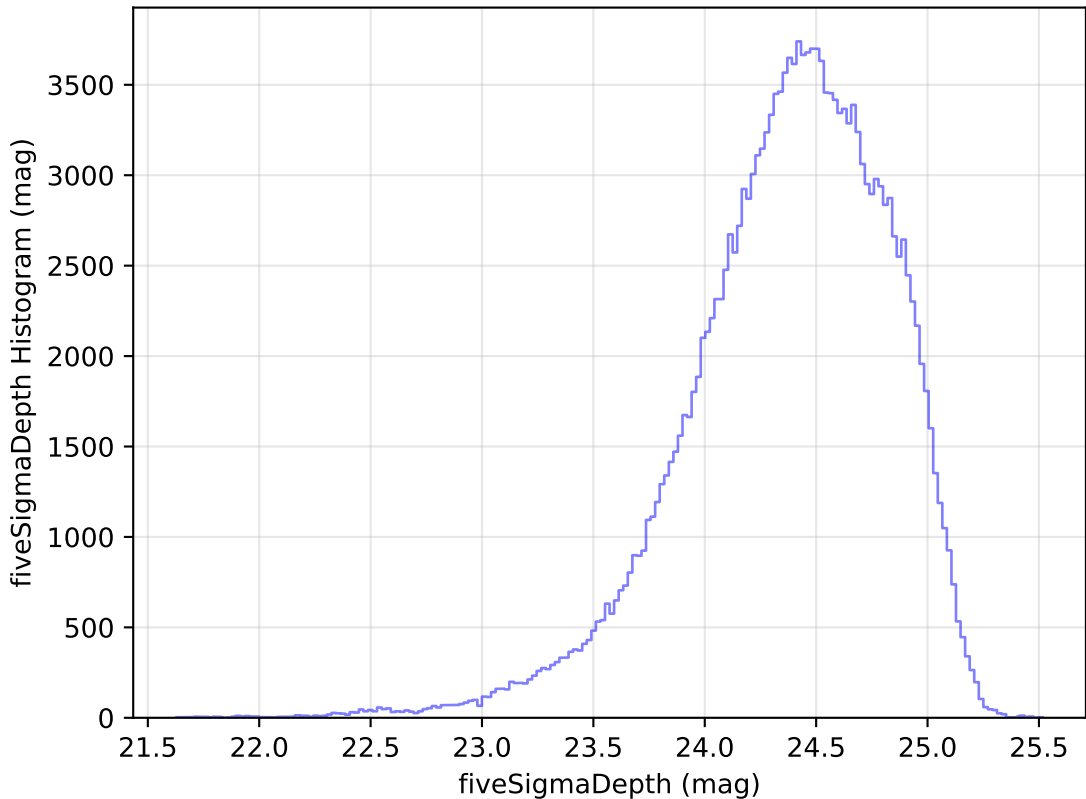
internal_u_expt38_nscale1.2v3.4_10yrs g: fiveSigmaDepth Histogram
